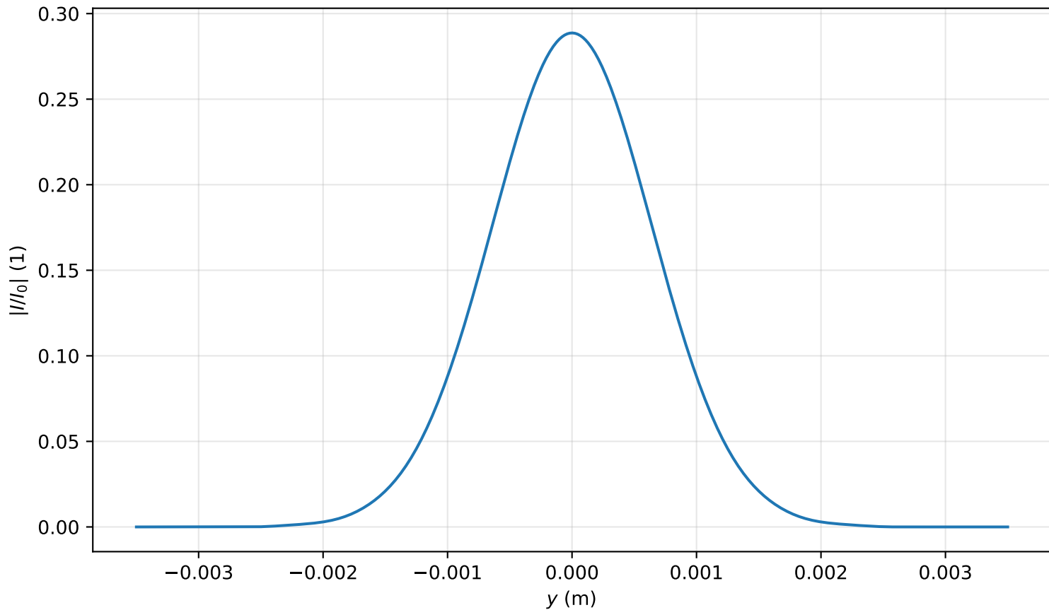
Intensity profile I(x=0, y, z=3.344)/I_0 , P_{in}=0.1P_{cr} , artificial time
